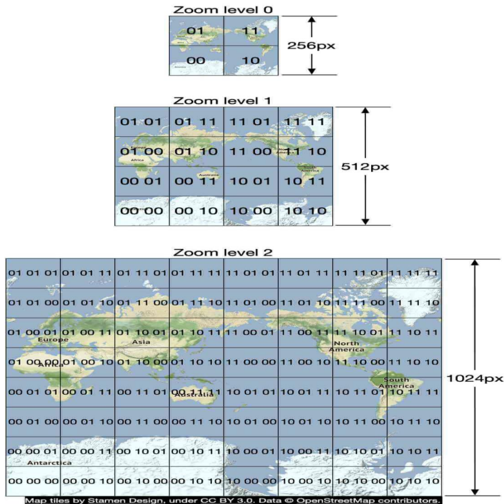
Figure 16 Zoom levels
