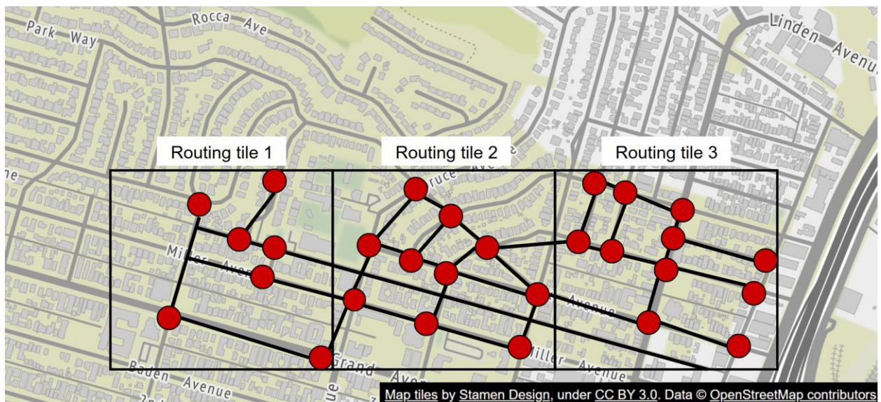
Figure 5 Routing tiles
