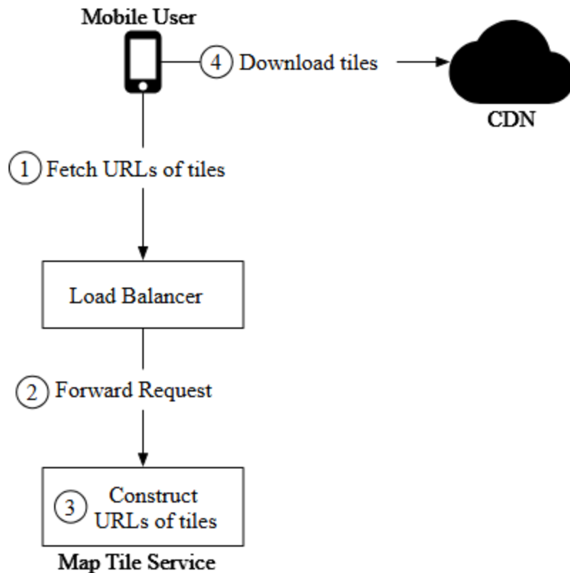
Figure 12 Map rendering
