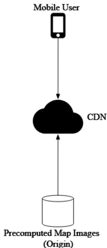
Figure 10 CDN
