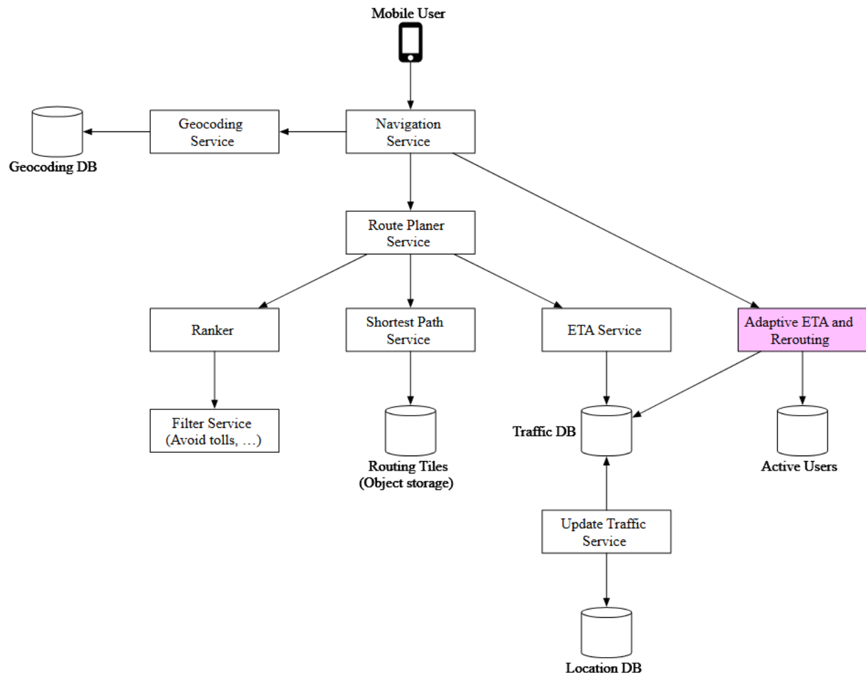
Figure 21 Final design
