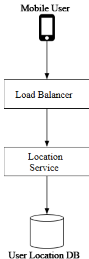
Figure 8 Location service
