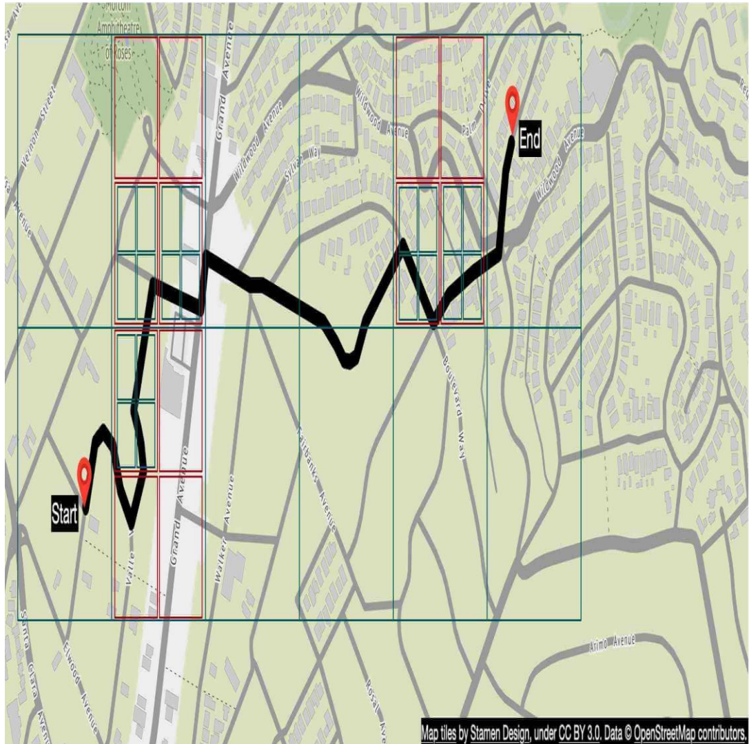
Figure 18 Graph traversal
