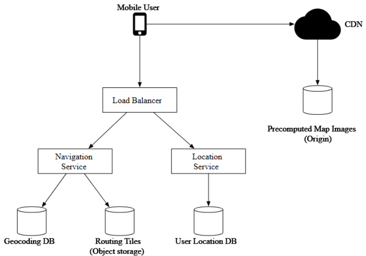
Figure 7 High-level design
