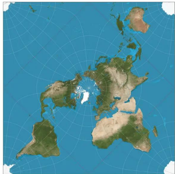
Peirce quincuncial projection
