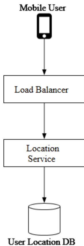
Figure 14 User location database
