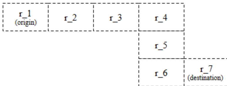
Figure 19 Navigation route
