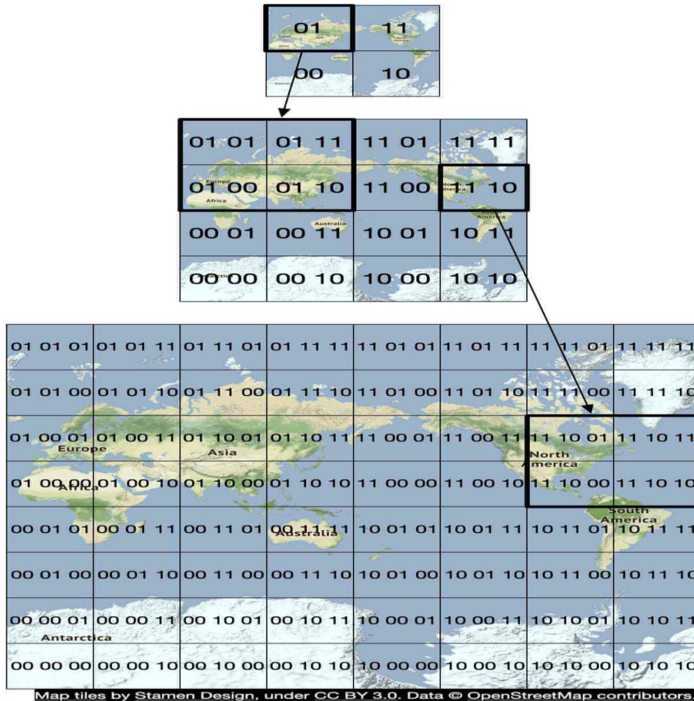
Figure 3 Geohashing
