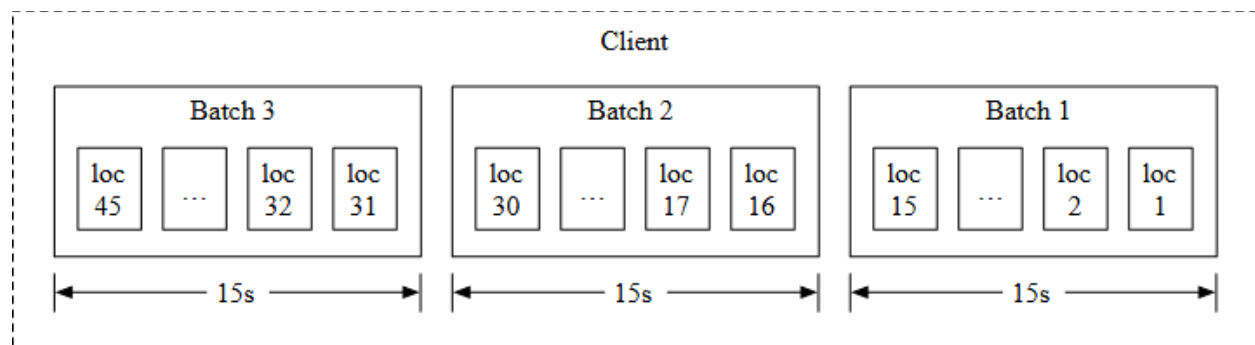
Figure 9 Batch requests
