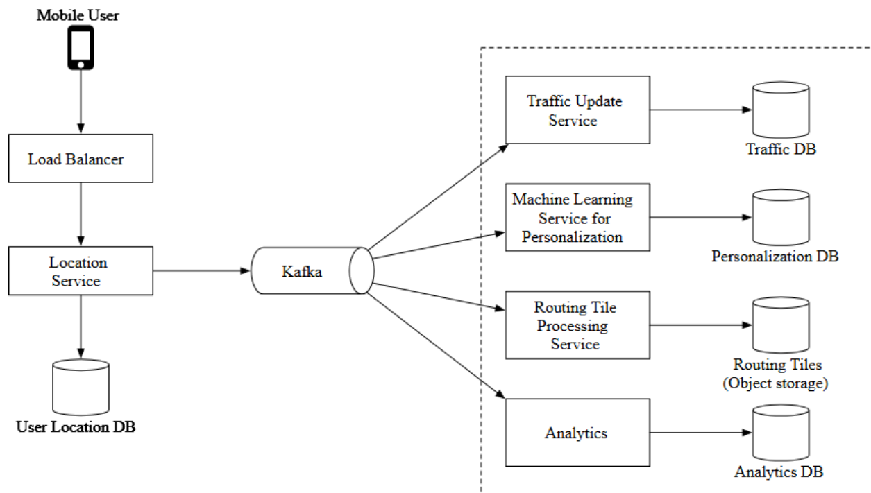
Figure 15 Location data is used by other services
